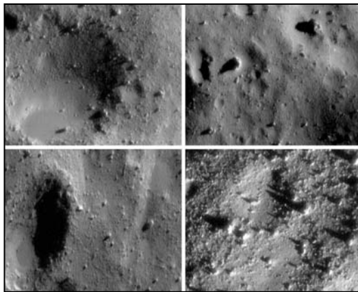
These images of Eros show the closest views of an asteroid ever seen. The top images are 550 m across, and the bottom images are 230 m across. The surface is dominated by small boulders.
