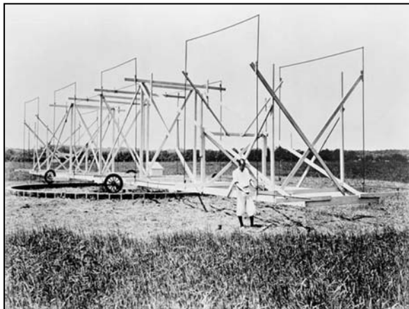
Karl Jansky with the first radio telescope, Holmdel, New Jersey.
