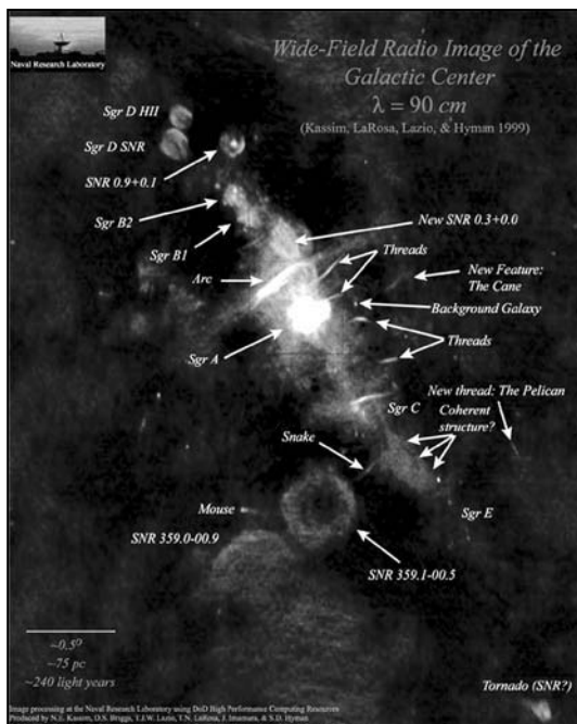
Image of our Galaxy, the Milky Way, as seen with the Very Large Array at 90 cm.
