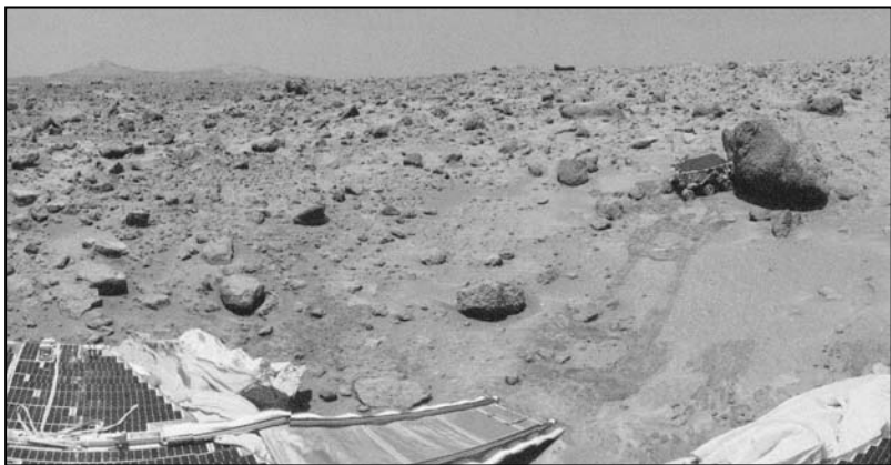
Section of a geometrically improved, color-enhanced version of a 360-degree pan taken by the Imager for Mars Pathfinder during 3 Martian days in 1997. Note Sojourner rover vehicle and its tracks.
